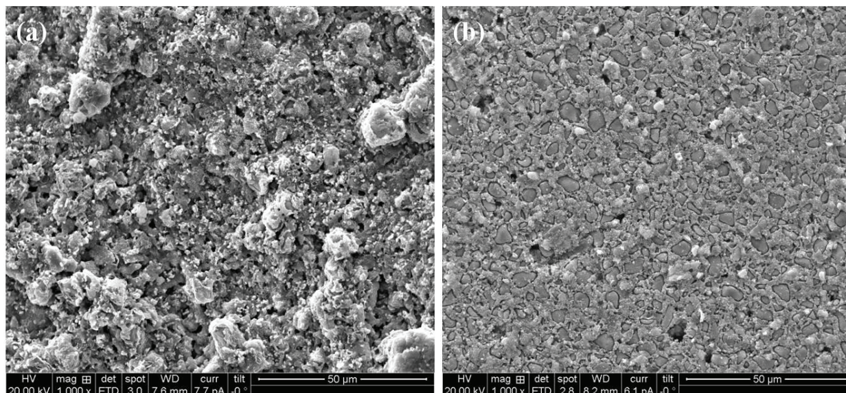
Figure 3: Scanning electron microscopic micrographs of self-etch primer- treated MTA Plus and Biodentine surfaces (a) MTA Plus- Selective loss of superficial globular structure with formation of porous surface (1000x) (b) Biodentine- Selective loss of crystalline appearance with formation of hexagonal microstructure (1000x)
