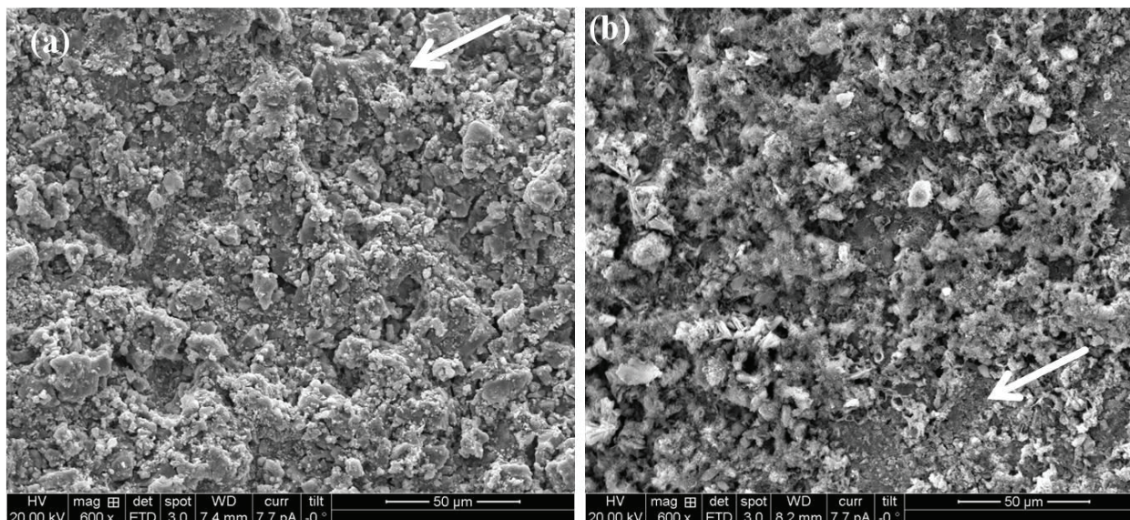
Figure 1: Scanning electron microscopic micrographs of untreated MTA Plus and Biodentine surfaces (a) Untreated MTA Plus surface with dense globular microstructure; bright white particles representing radiopacifier phase (arrowheads) (600x) (b) Untreated Biodentine surface with less intense globular microstructure; needle-like crystalline appearance (arrowheads) (600x)
