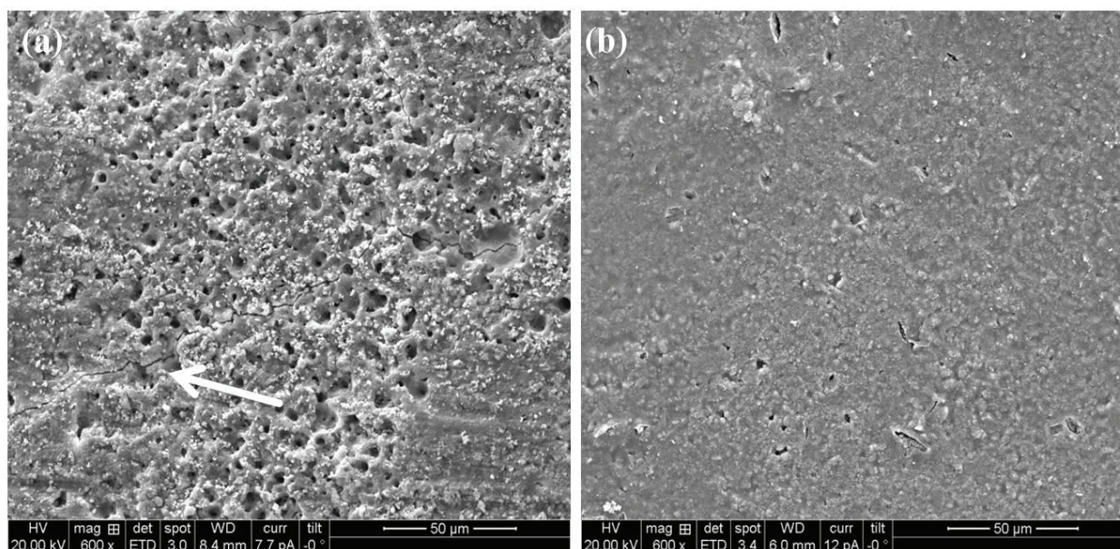
Figure 2: Scanning electron microscopic micrographs of phosphoric acid-treated MTA Plus and Biodentine surfaces (a) MTA Plus - Severe loss of globular structure with formation of deep pores and cracks (arrowheads) (600x) (b) Biodentine- Loss of globular structure with formation of pores; loss of crystalline appearance (600x)
